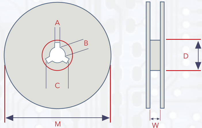
REEL DIMENSION (MM)
